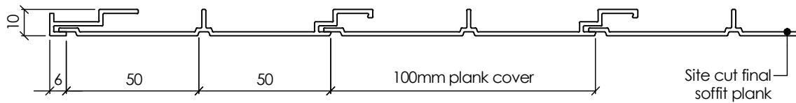
Assembly Profile (1:2)
