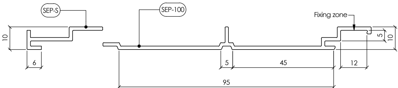
Component Details (1:1)
