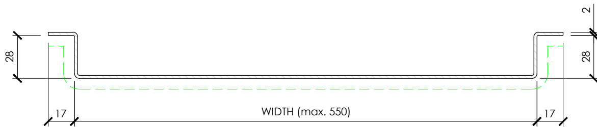
PANEL PROFILE
