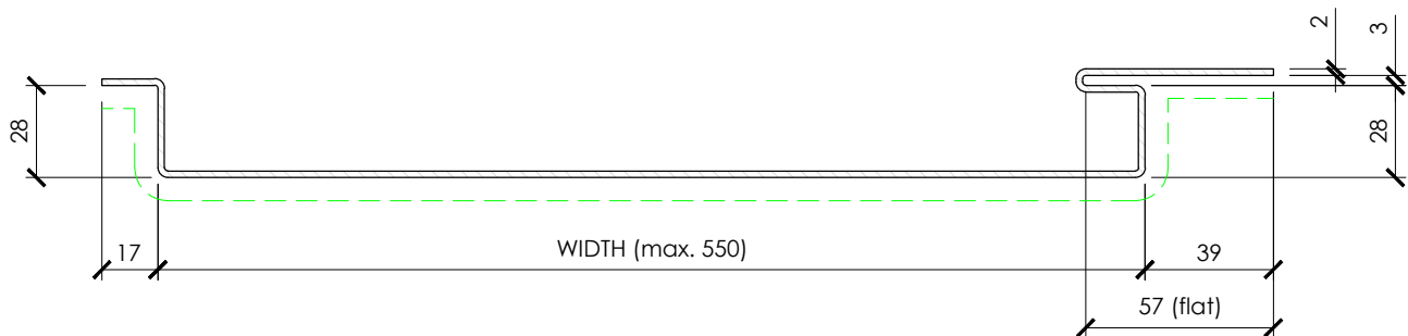
PANEL PROFILE
