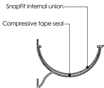
Section B-B Through Internal Union (1 : 4)
