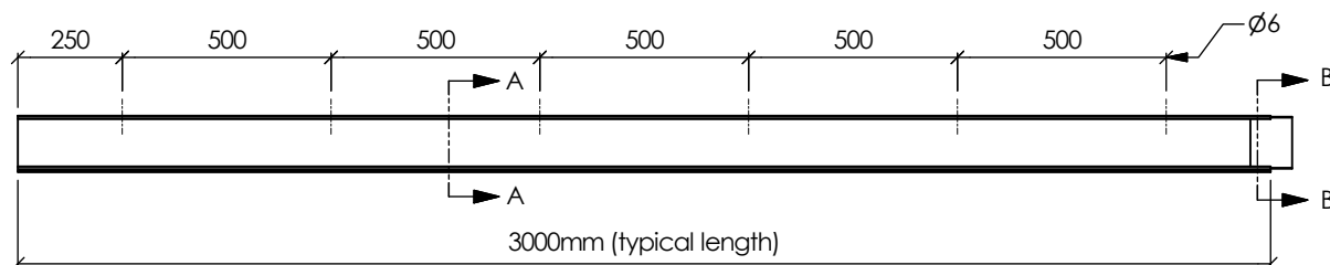
View on Plan (1 : 20)
