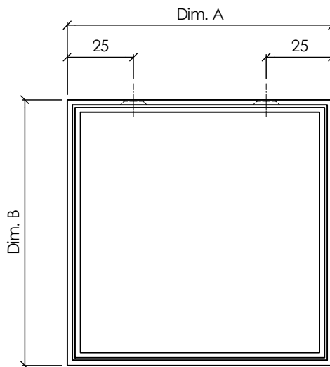
VIEW ON PLAN ( 1 : 2 )
