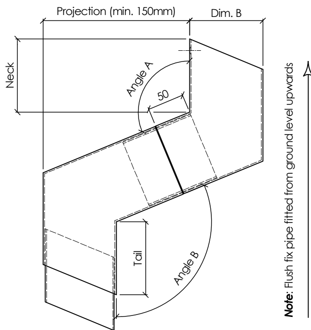
SIDE VIEW ( 1 : 5 )
