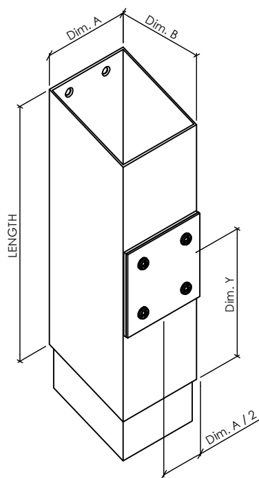
ISOMETRIC VIEW
