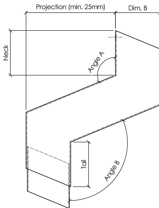
SIDE VIEW ( 1 : 5 )
