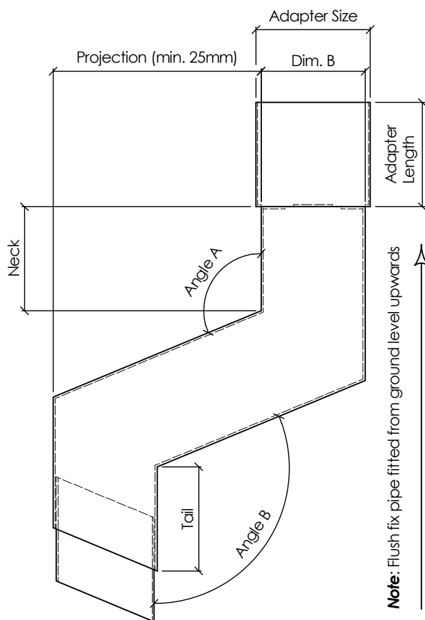
SIDE VIEW ( 1 : 5 )
