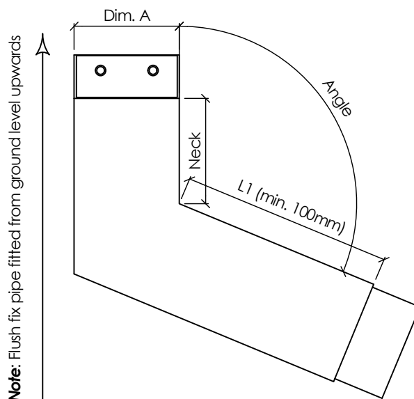
FRONT VIEW ( 1 : 5 )
