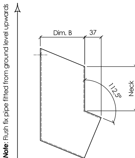
SIDE VIEW ( 1 : 5 )
