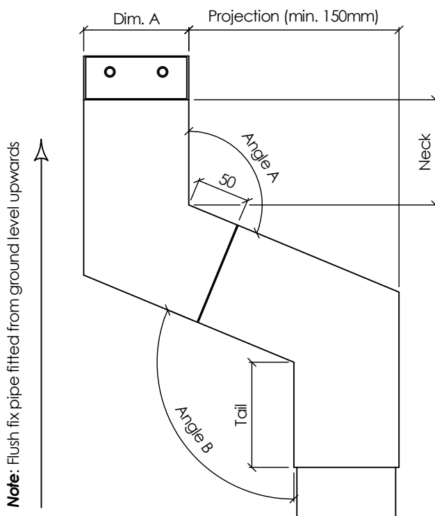
FRONT VIEW ( 1 : 5 )
