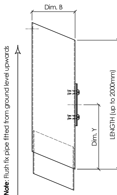
SIDE VIEW ( 1 : 5 )
