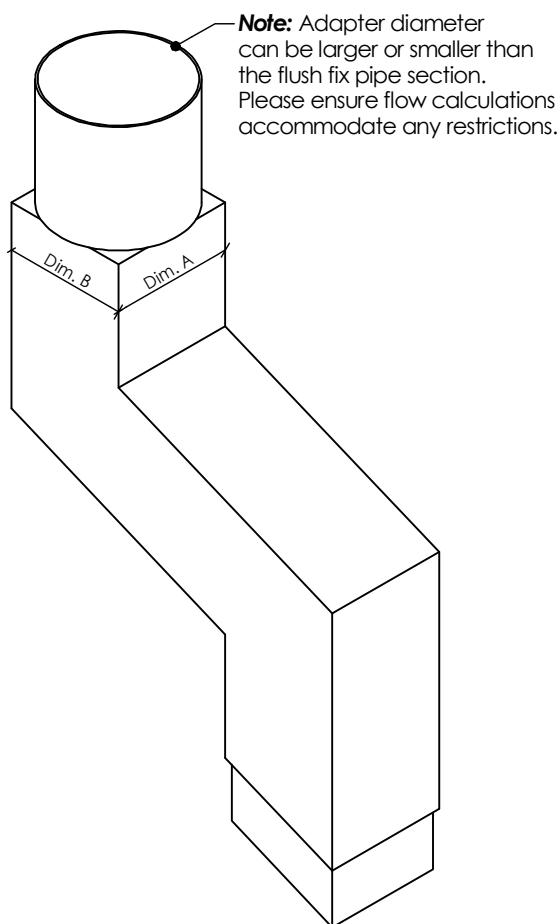
ISOMETRIC VIEW
