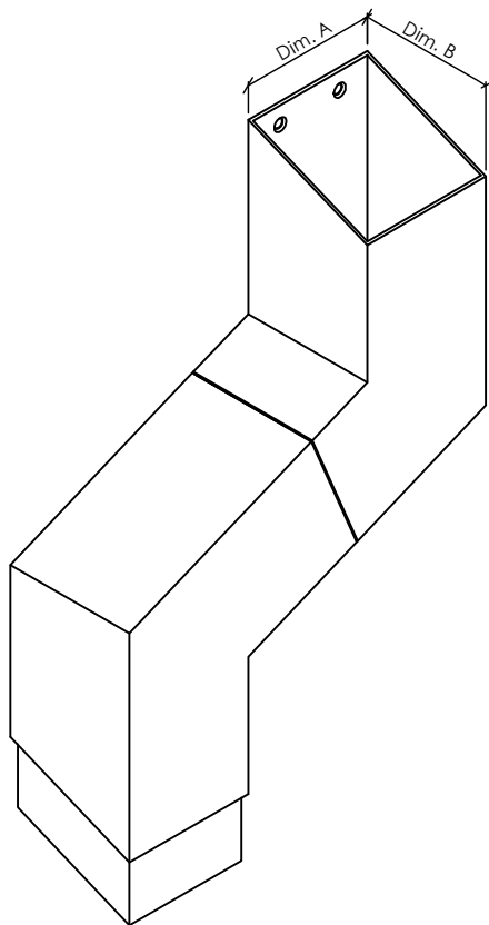
ISOMETRIC VIEW
