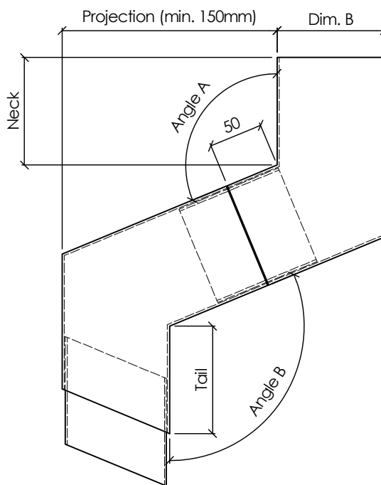
SIDE VIEW ( 1 : 5 )
