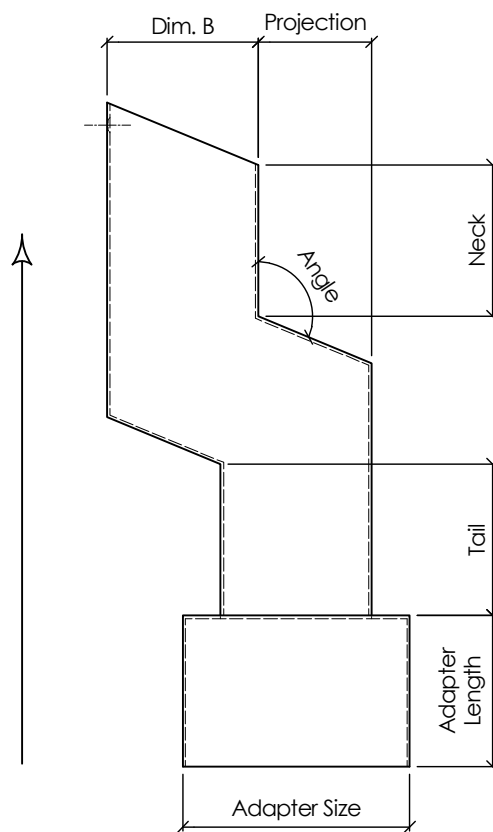
SIDE VIEW ( 1 : 5 )
