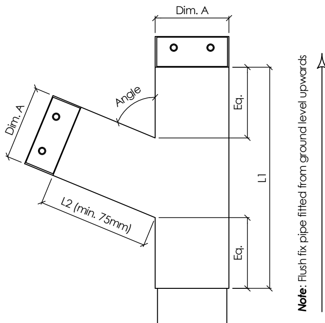
FRONT VIEW ( 1 : 5 )
