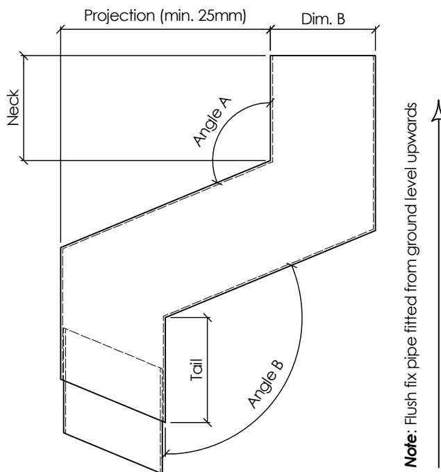
SIDE VIEW ( 1 : 5 )
