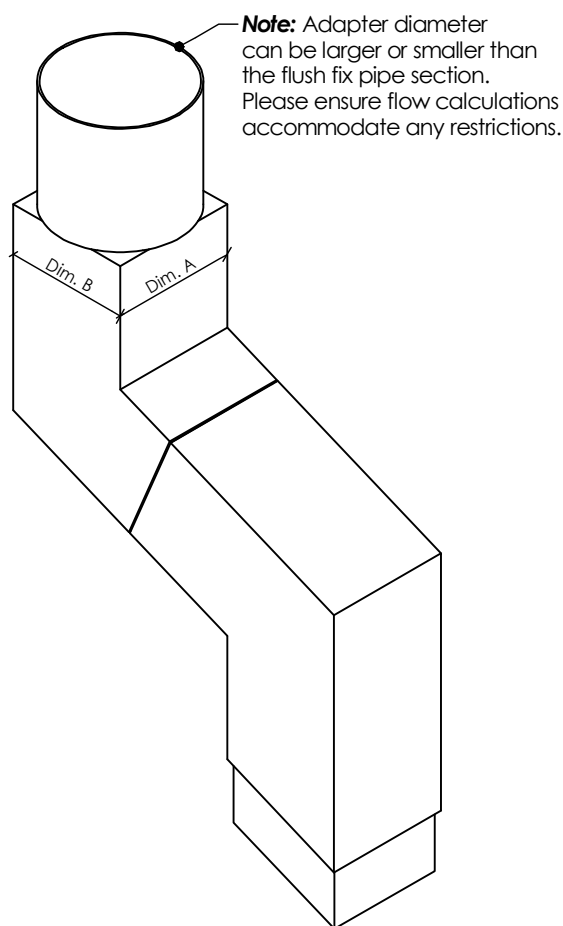
ISOMETRIC VIEW
