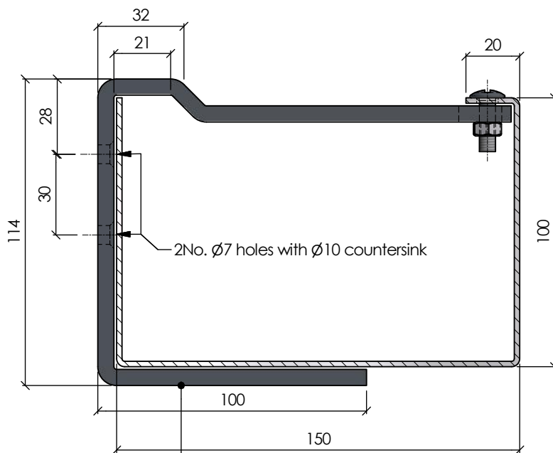
Section A-A (1:2)
