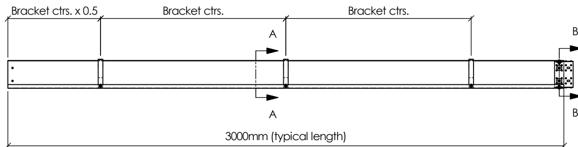
View on Plan (1:20)
