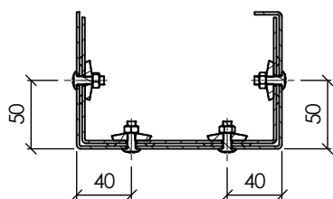
Section B-B Union Hole Locations (1:5)
