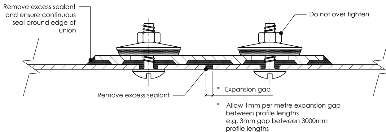
SECTION THROUGH STANDARD GUTTER JOINT
