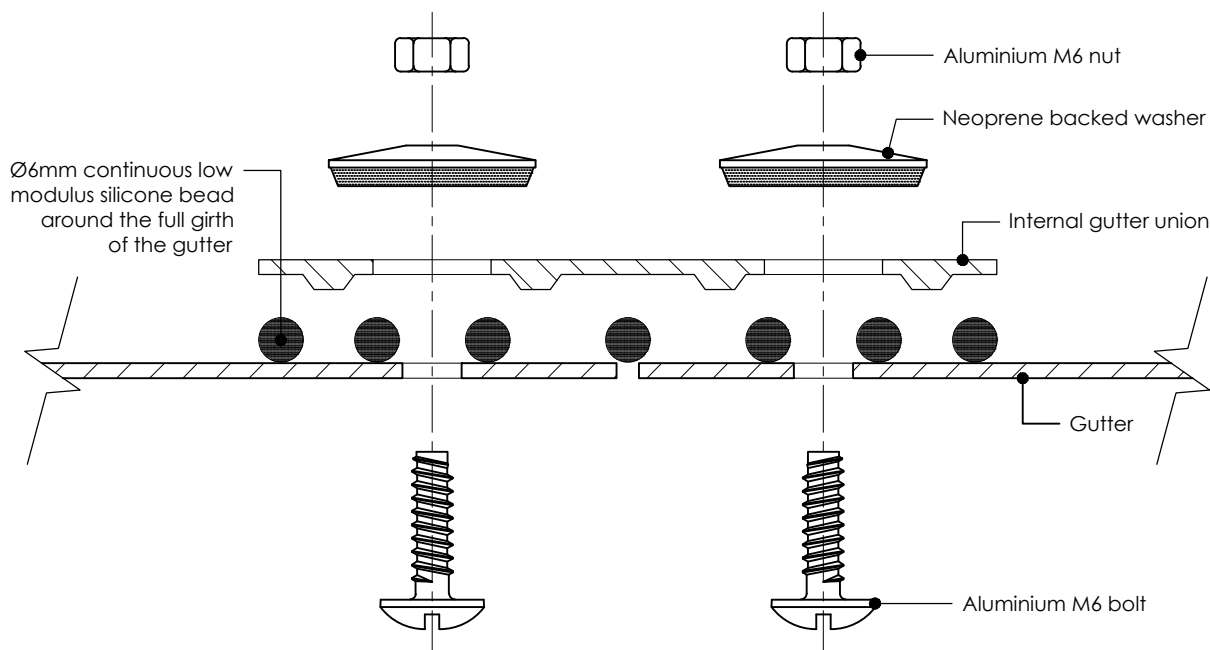
EXPLODED GUTTER JOINT ASSEMBLY
