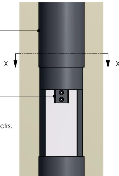
View on Front Elevation at Pipe Joint (1:5)
