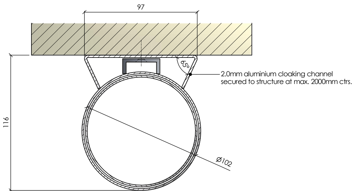
Section X-X (1:2)
