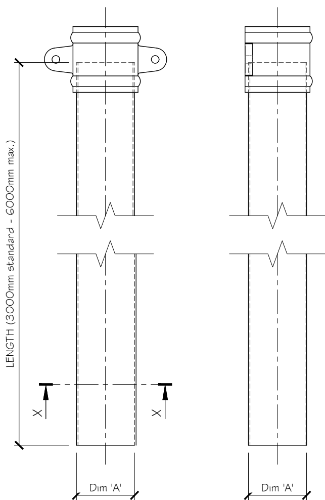
VIEW ON ELEVATION
