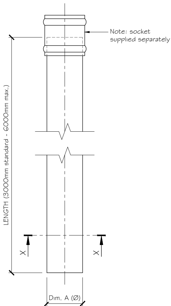
VIEW ON ELEVATION
