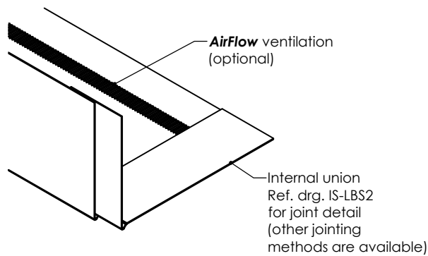
Isometric View
