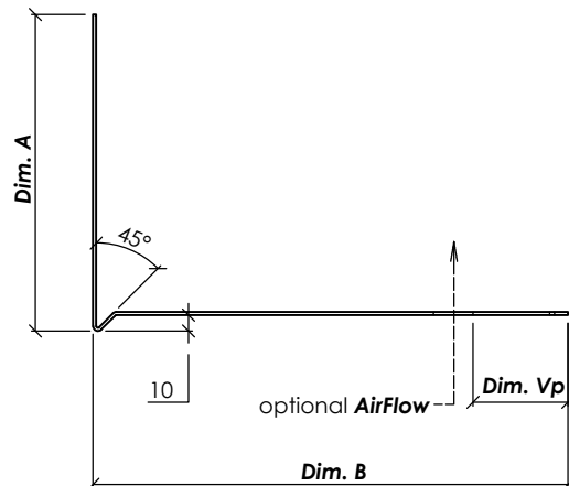
Profile Section (1 : 5)
