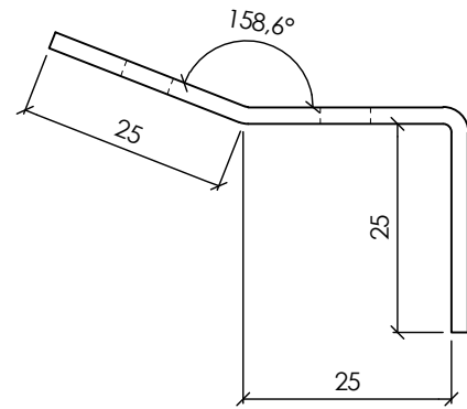
COLUMN CASING SUPPORT PROFILE A (1:1)
