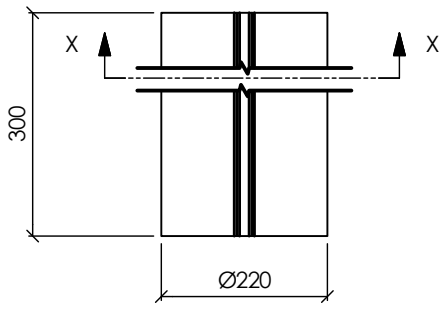
VIEW ON ELEVATION (1:10)
