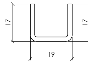
JOINT COVER PROFILE (1:1)
