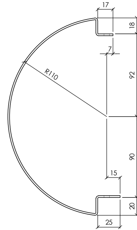
COLUMN CASING PROFILE (1:2.5)
