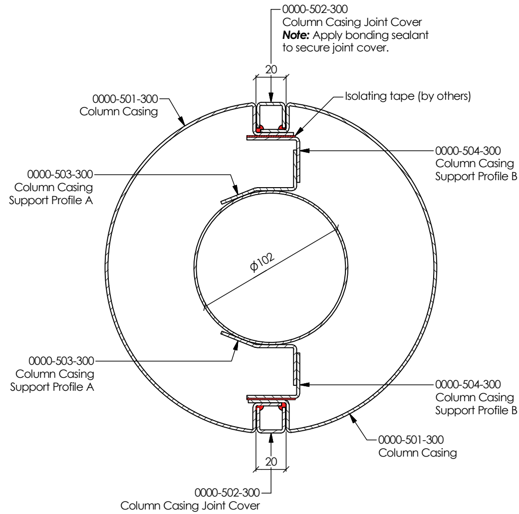
SECTION X-X (1:2.5)
