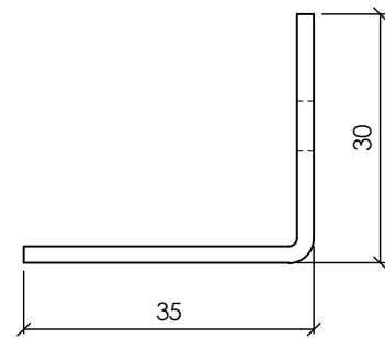
COLUMN CASING SUPPORT PROFILE B (1:1)
